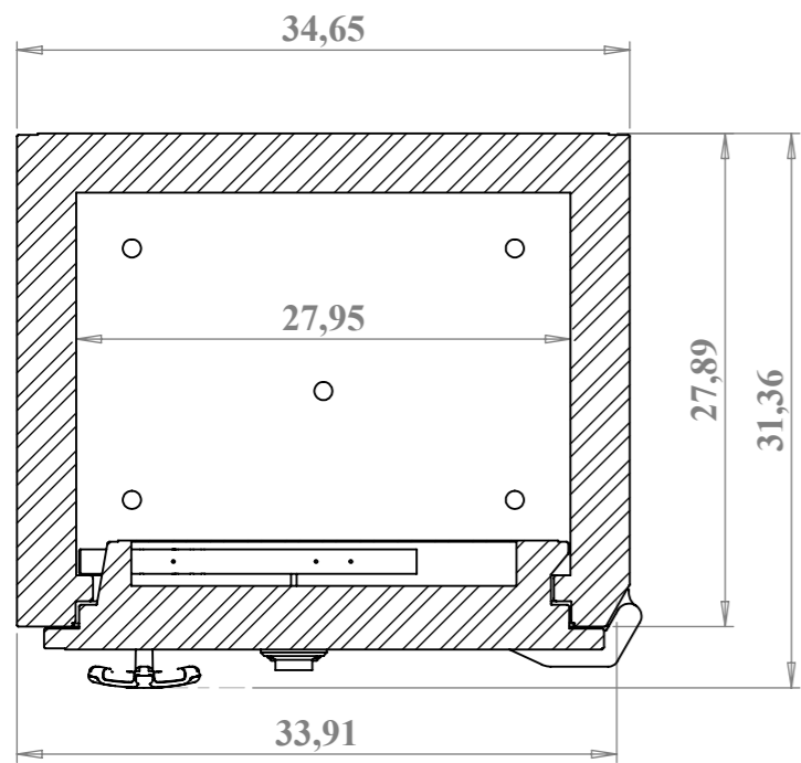
F-F (1 : 12) 19,69
