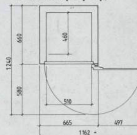
PLAN 204, 5, 6, 7
