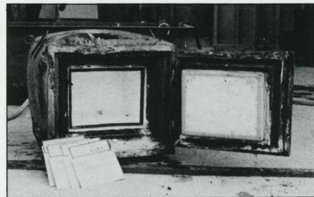
The MVP-101 after testing — While the outside is charred and swollen from heat, both the media storage area and data contained on the diskettes remained intact.
